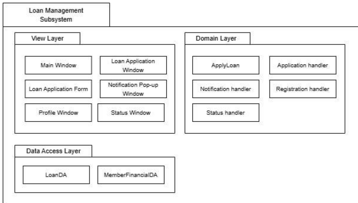
Figure 4.2.4: Package Diagram for <Loan Management> Subsystem
