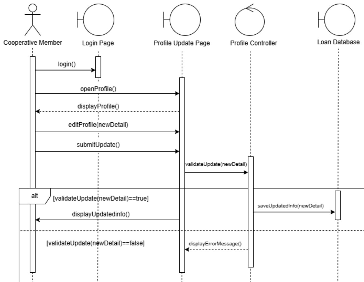
Figure 4.4.6: SD006 Sequence Diagram for <Manage Profile>
