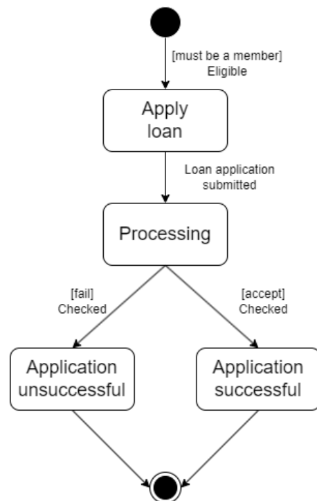
Figure 2.2.3: State Diagram for Loan Application Koperasi KADA Online System
