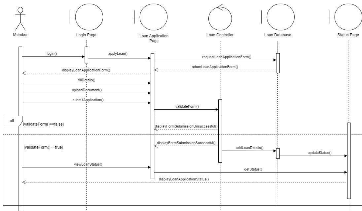
Figure 4.4.5: SD005 Sequence Diagram for <View Loan Application Status>
