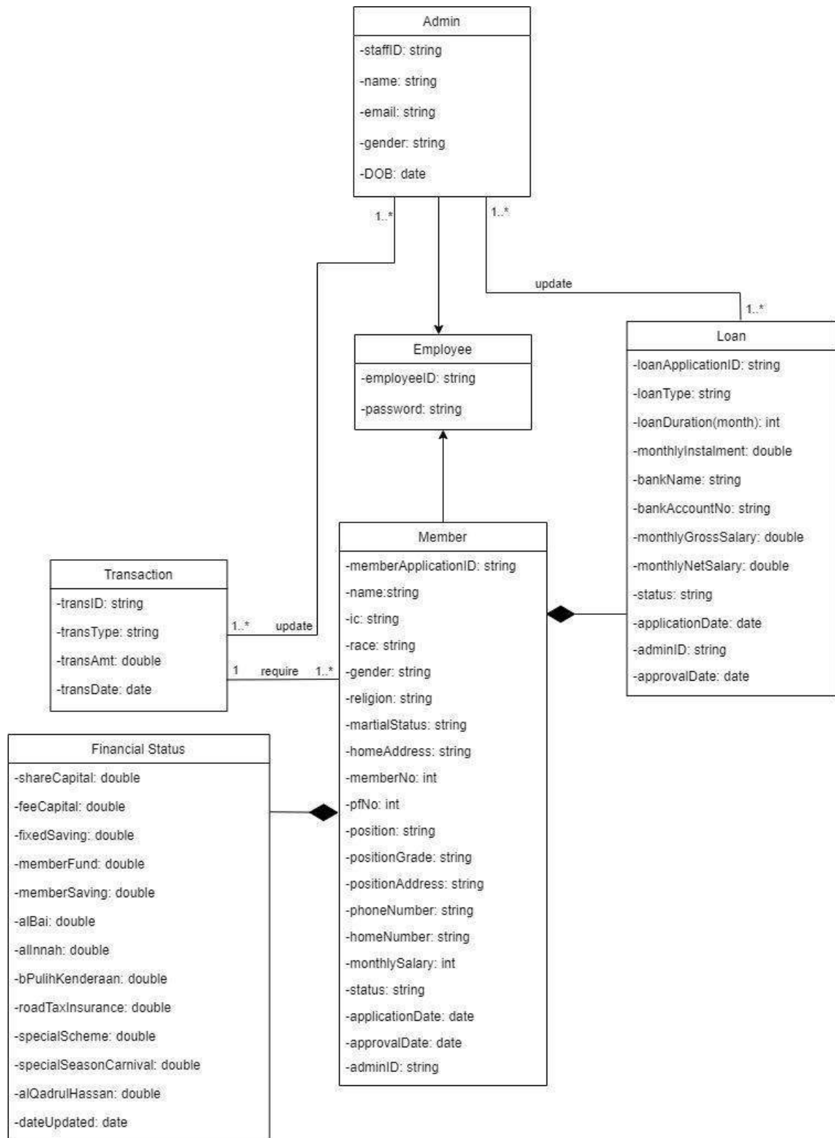
Figure 4.3.3: Class Diagram for <View Financial Status> Subsystem
