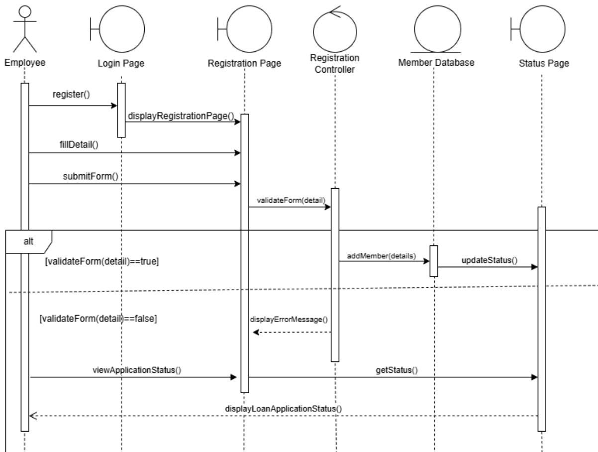
Figure 4.4.1: SD001 Sequence Diagram for <Apply Membership>
