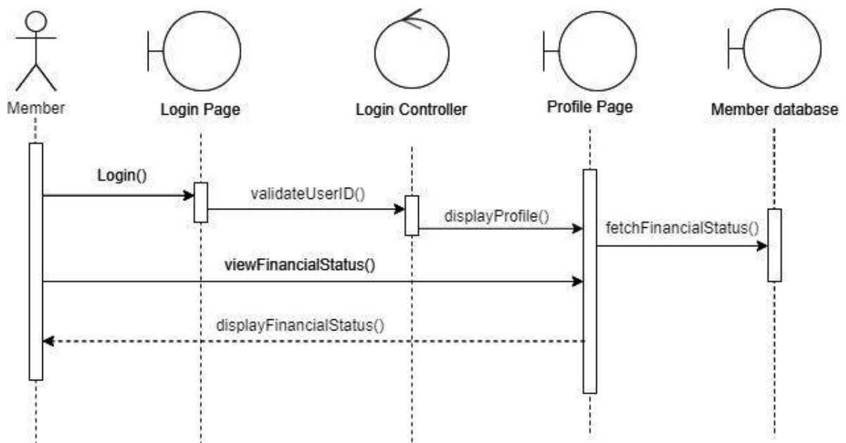
Figure 4.4.3: SD003 Sequence Diagram for <View Financial Status>
