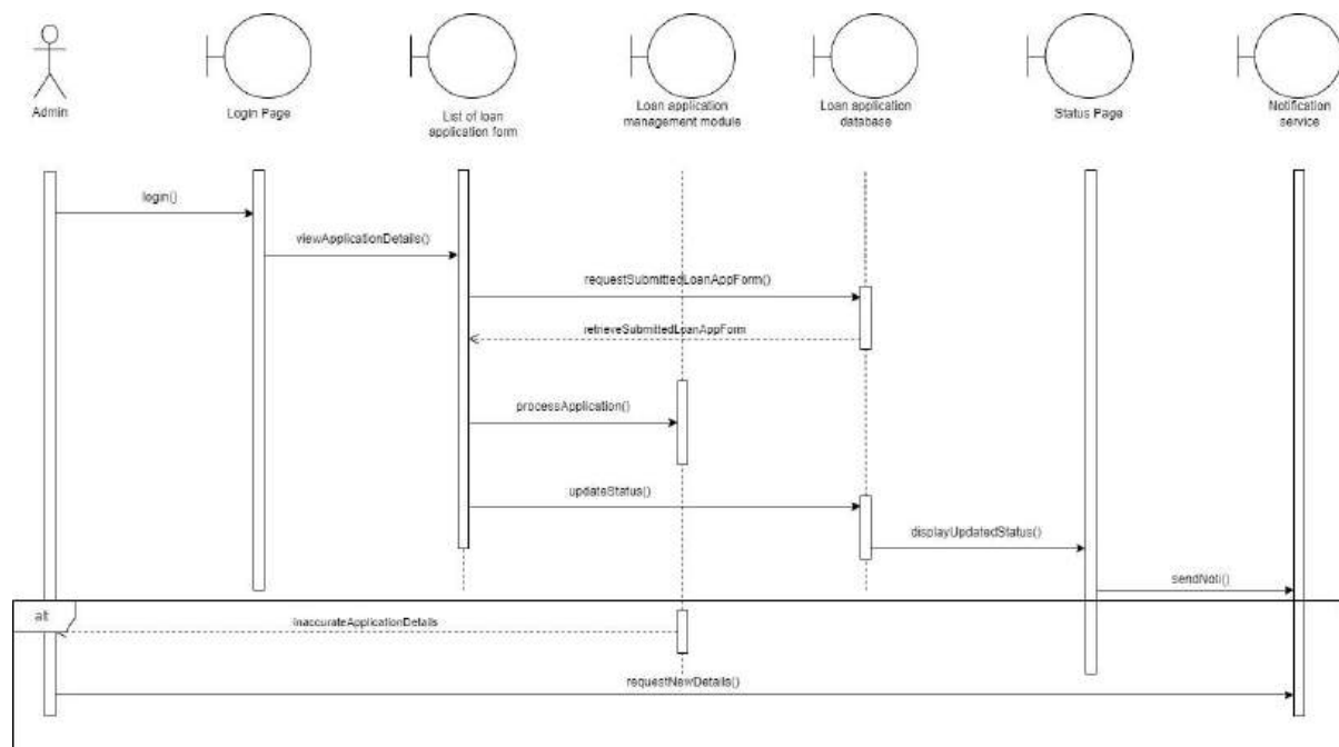
Figure 2.4.9.2: Sequence Diagram for Approve Loan Application
