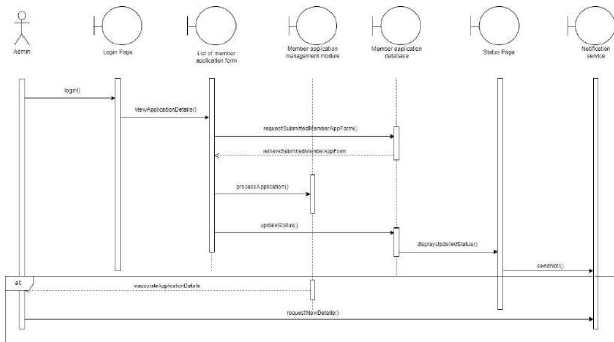
Figure 4.4.8: SD008 Sequence Diagram for <Approve Membership Application >
