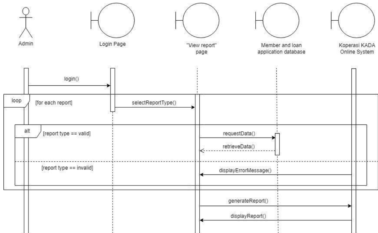
Figure 4.4.11: SD0011 Sequence Diagram for < Generate Report>
