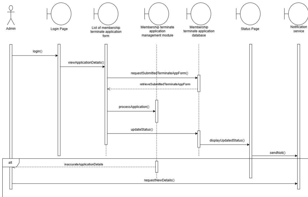
Figure 4.4.10: SD009 Sequence Diagram for <Approve Terminate Membership Application >
