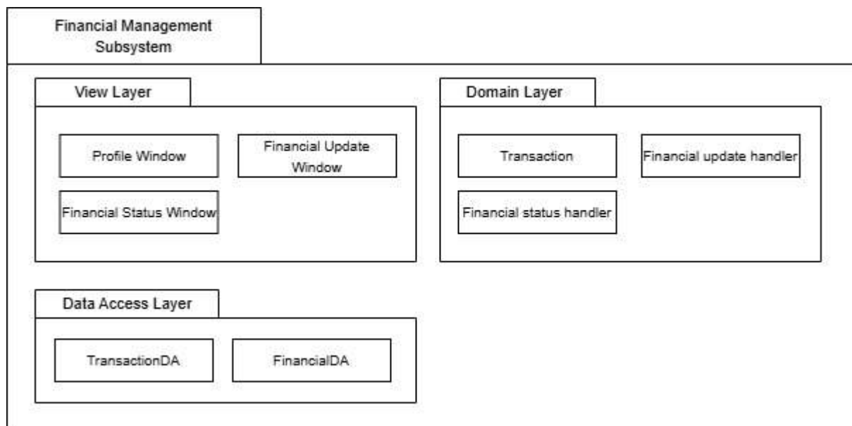
Figure 4.2.5: Package Diagram for <Financial Management> Subsystem
