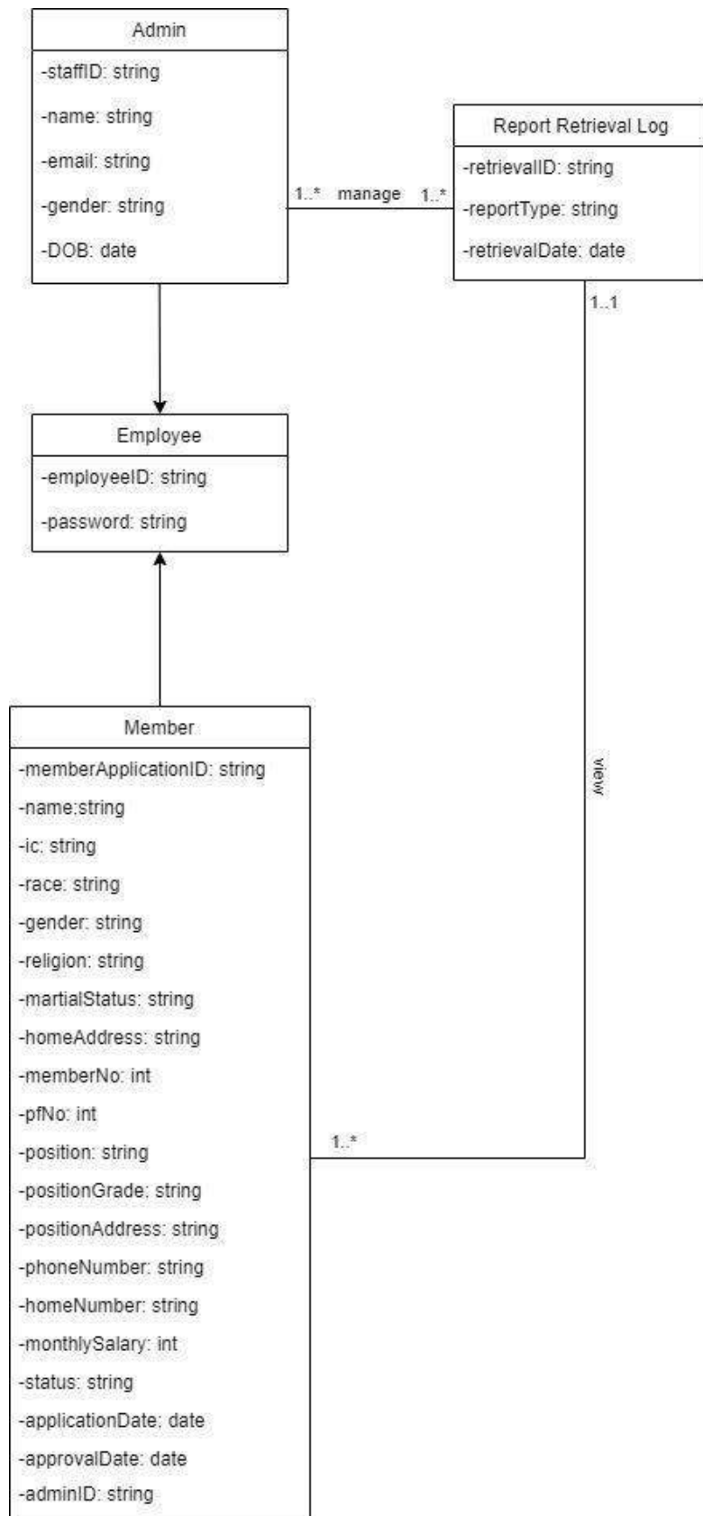
Figure 4.3.4: Class Diagram for <Process Report> Subsystem
