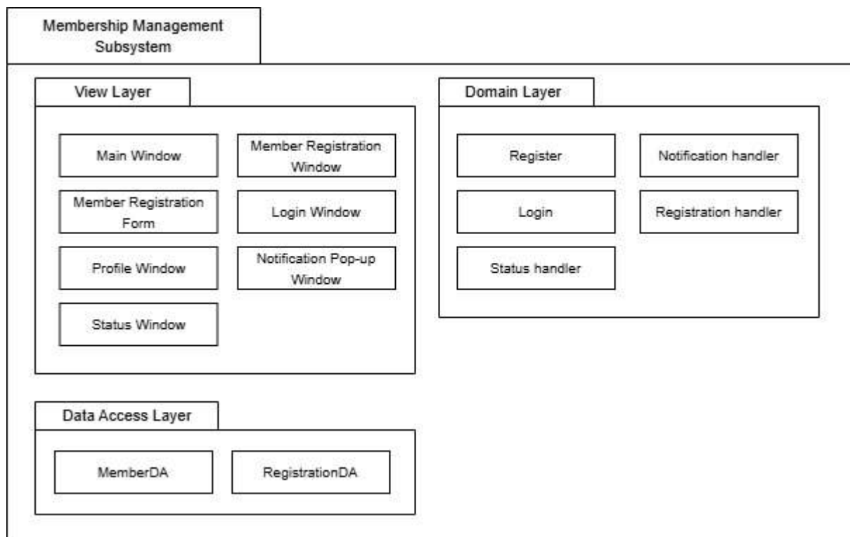
Figure 4.2.3: Package Diagram for <Membership management> Subsystem
