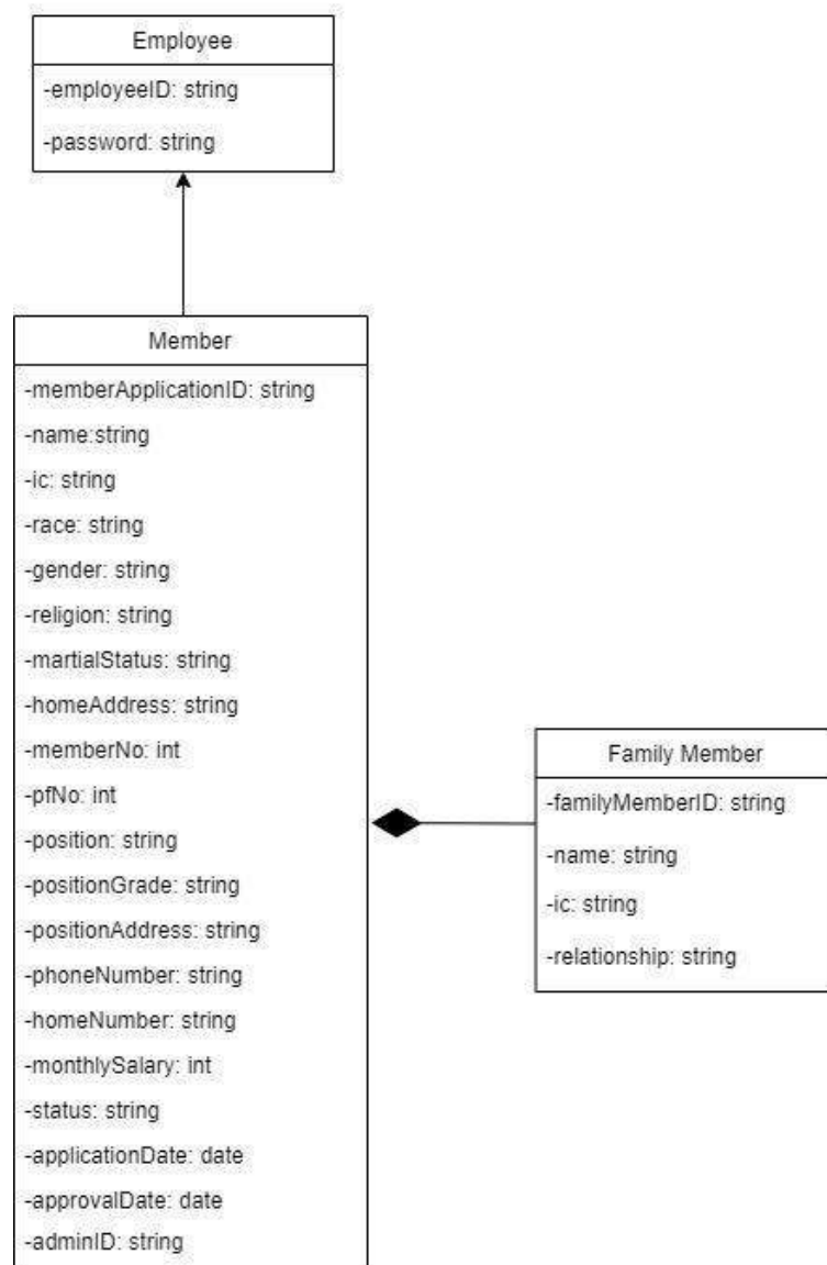
Figure 4.3.1: Class diagram for <Apply for Membership> Subsystem
