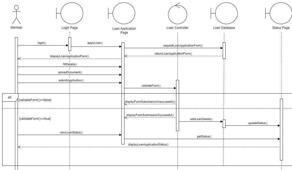
Figure 4.4.4: SD004 Sequence Diagram for <Apply for Loan>
