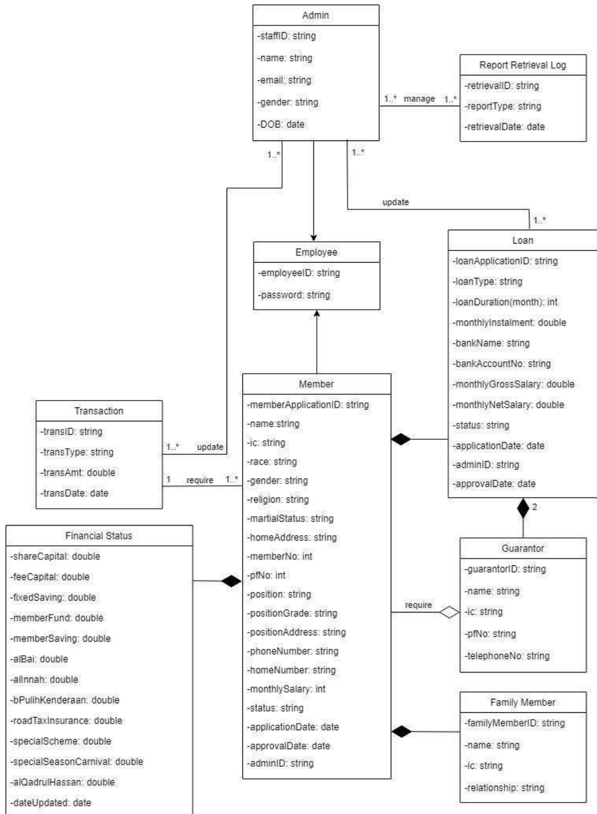
Figure 4.3.5: Class Diagram for <Koperasi KADA Online System> Subsystem
