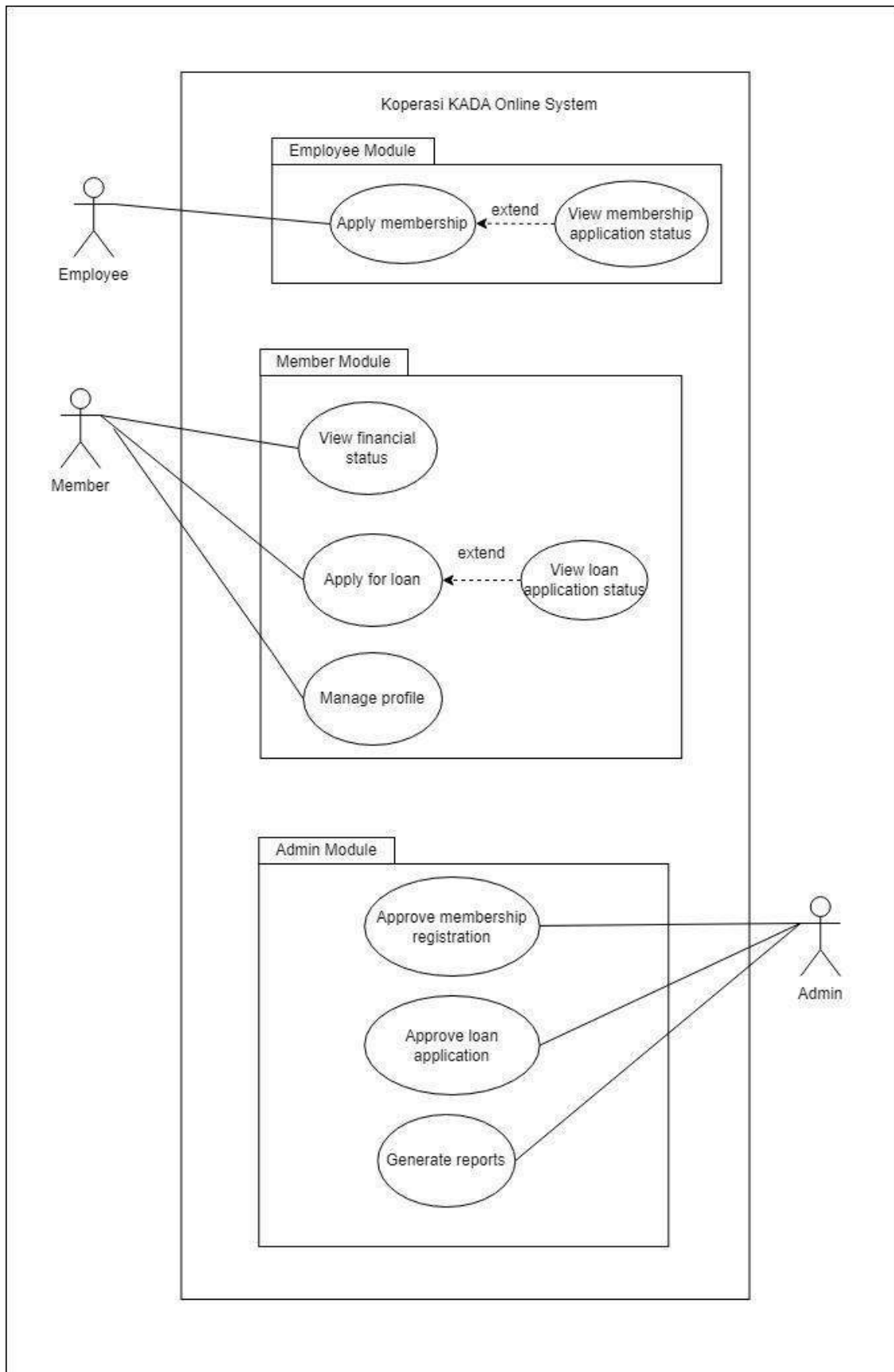
Figure 2.2.1: Use Case Diagram for Koperasi KADA Online System
