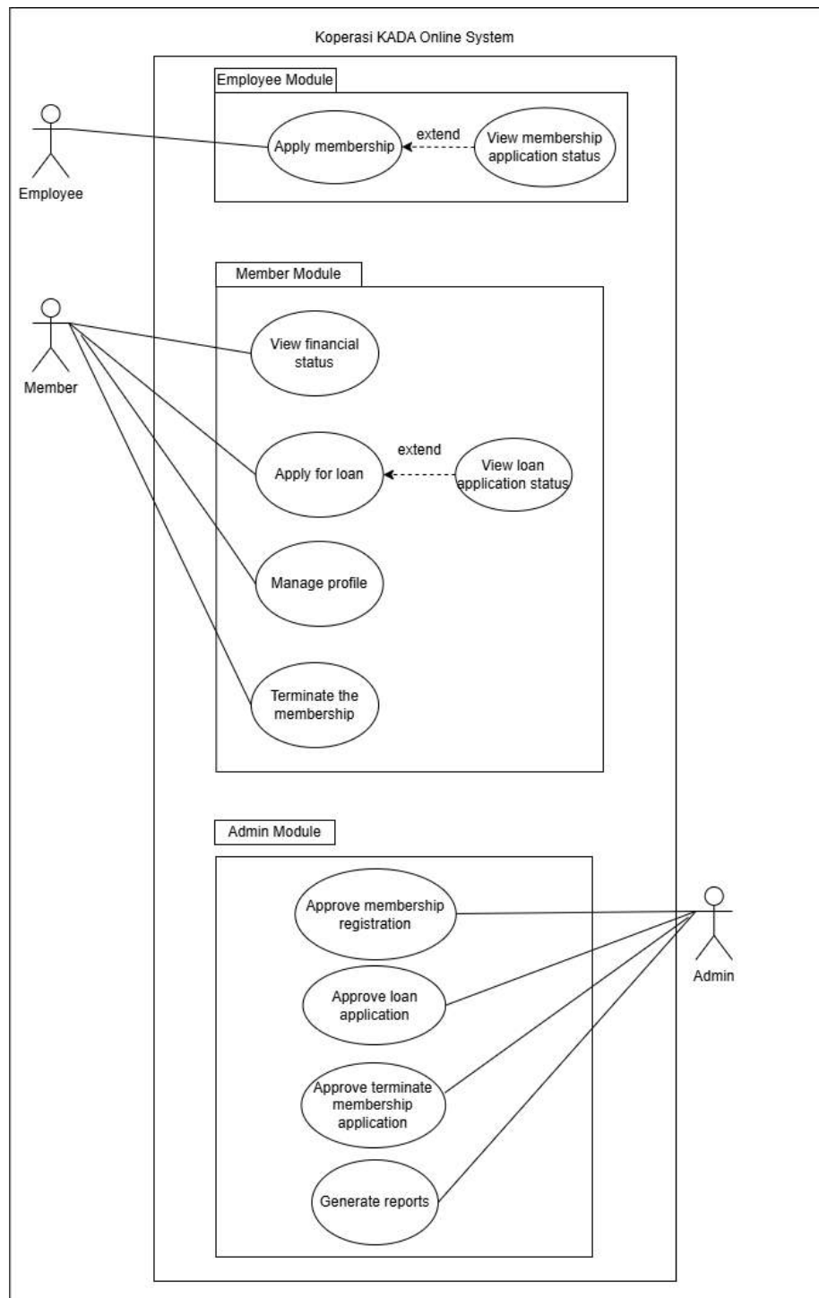
Figure 4.1.1: Use Case Diagram for <Koperasi KADA Online System>
