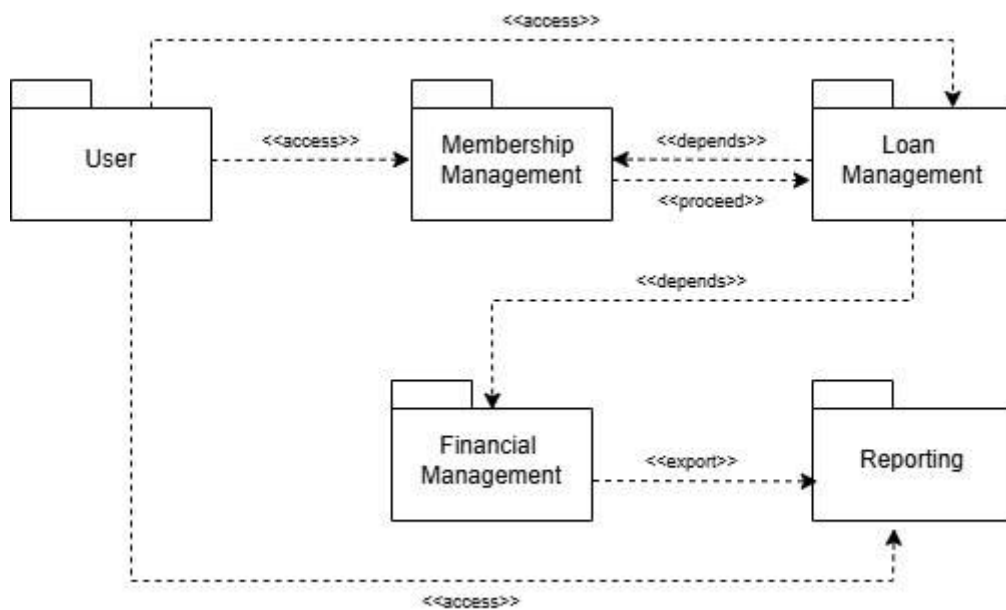
Figure 4.2.2: Package Diagram for <Koperasi KADA Online System>
