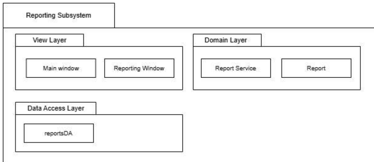
Figure 4.2.6: Package Diagram for <Reporting> Subsystem
