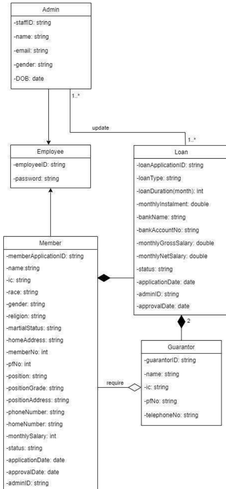
Figure 4.3.2: Class Diagram for <Apply for Loan> Subsystem
