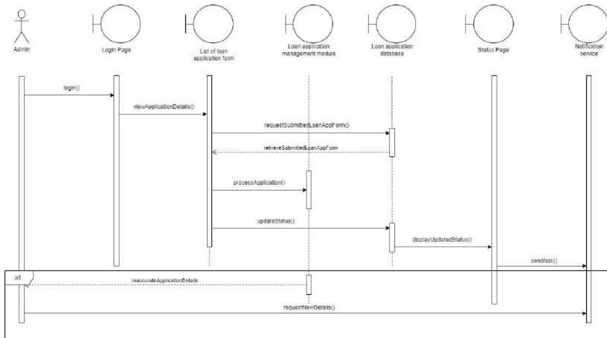
Figure 4.4.9: SD009 Sequence Diagram for <Approve Loan Application >
