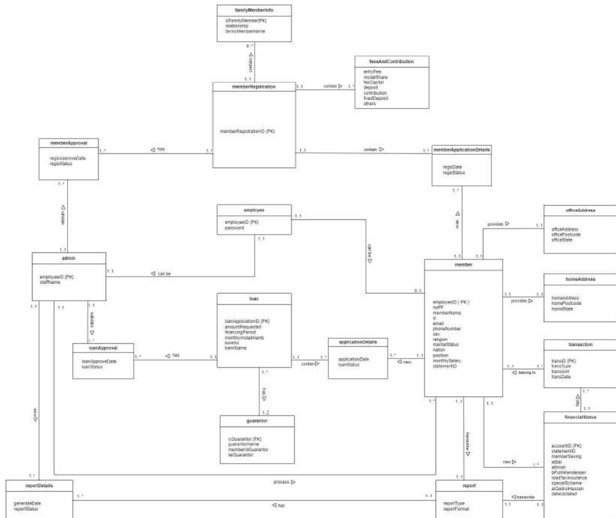
Figure 5.1 Logical ERD for Koperasi KADA Online System
