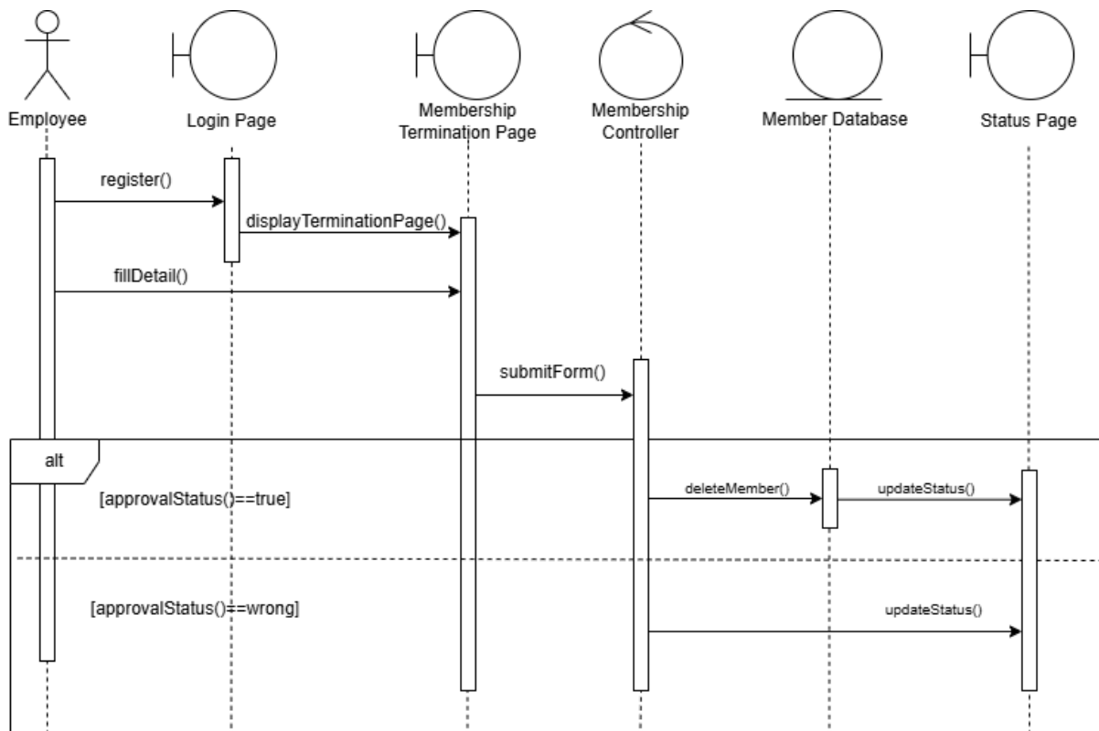
Figure 4.4.7: SD007 Sequence Diagram for <Terminate the Membership>
